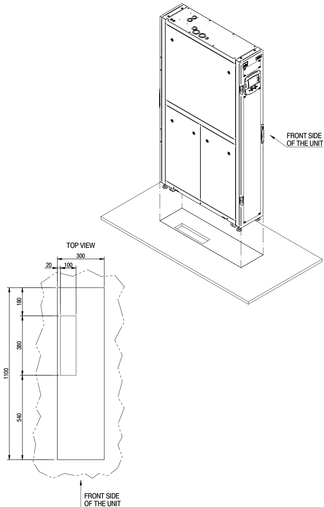
Fig. 8d Hole on the raised floor for piping - CW
