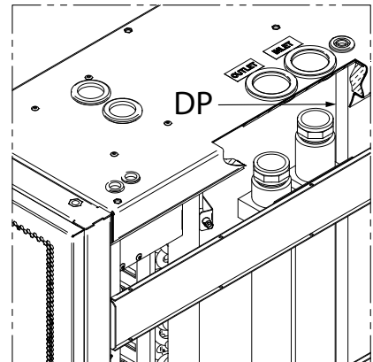
TOP CHILLED WATER CONNECTIONS
