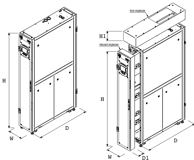
Fig. 8b Overall dimensions / service area
