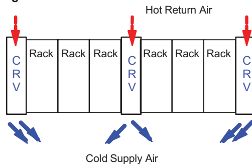
Fig. 2b Liebert® CRV – Single Row Placement
