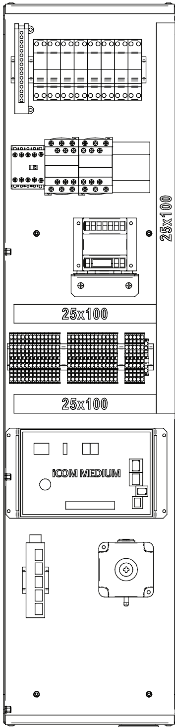
Fig. 9c CW electrical board layout
