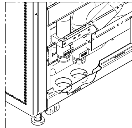
REAR BOTTOM CHILLED WATER CONNECTIONS
