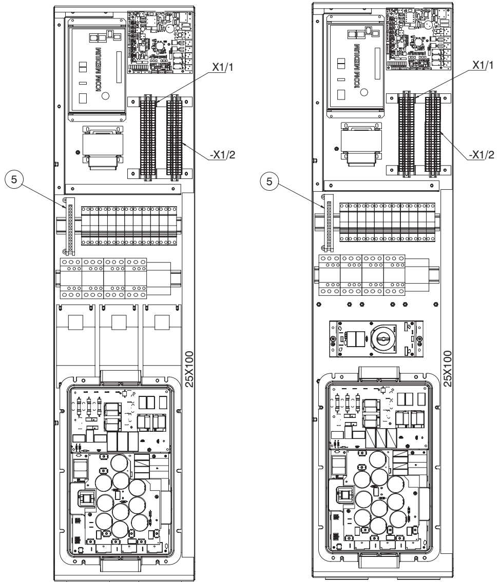
Fig. 9c DX electrical board layout
