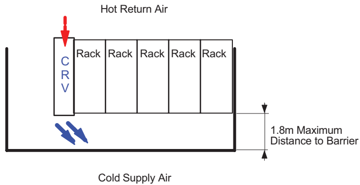
Fig. 2d Simulated aisle containment using room barriers – single row
