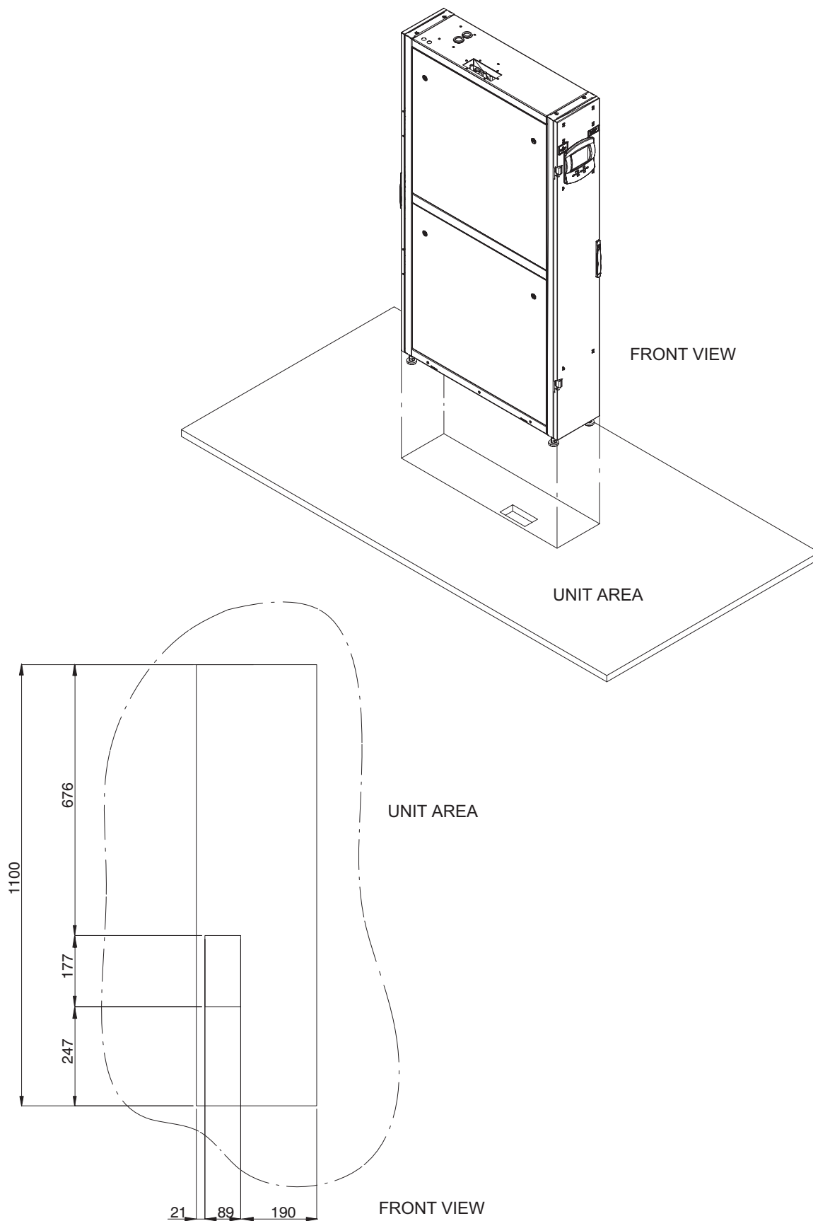
Fig. 8c Hole on the raised floor for piping - DX
