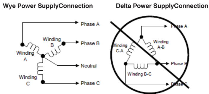
Fig. 6a Wye vs. Delta power supply connection diagram
