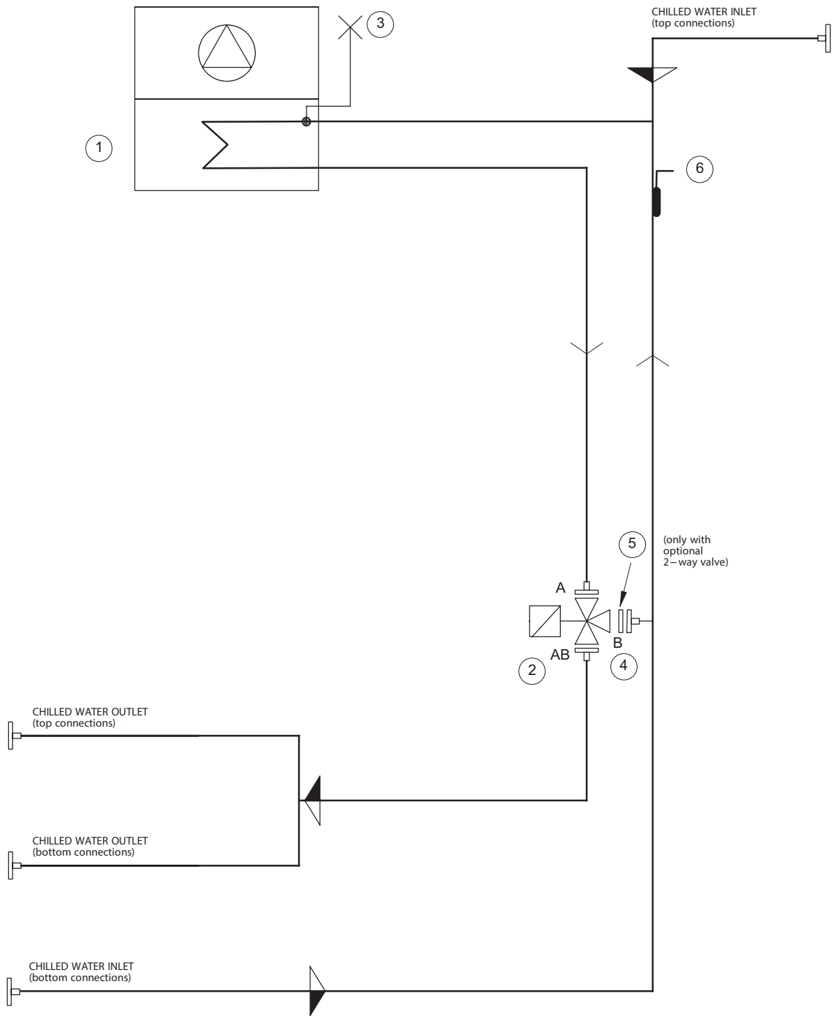
Fig. 10b Liebert CR032RC - CR060RC
