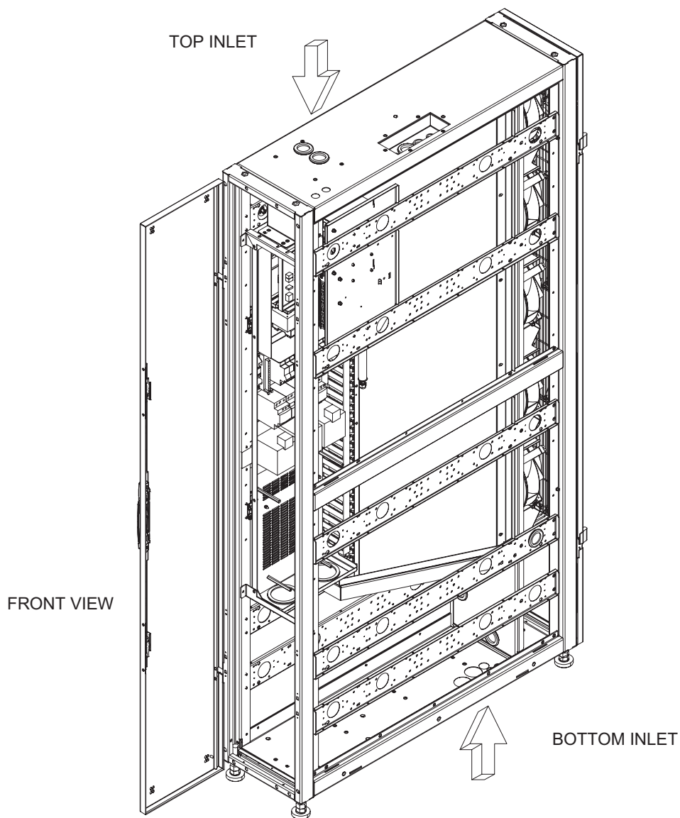
Fig. 8f Electrical connections - entry - DX
